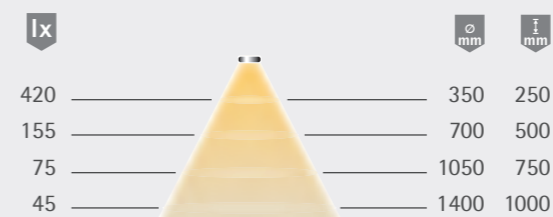
Light distribution diagram 70°
